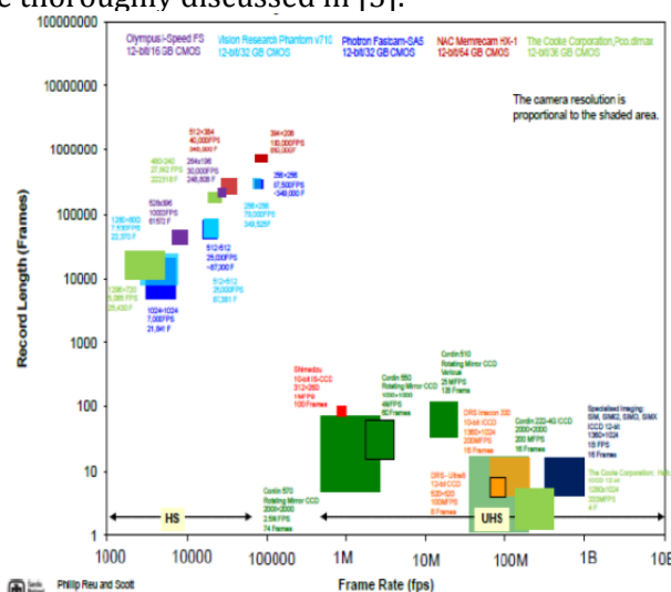
Figure 2: Summary of recent devices: record length vs frame rate & imager size
