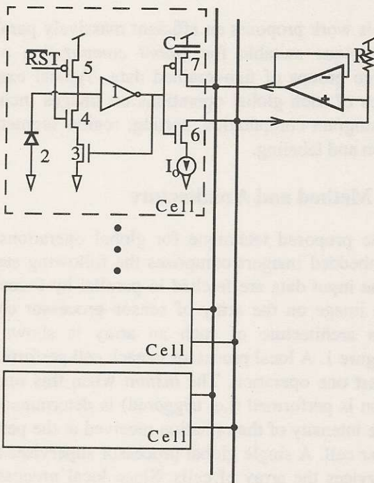
Figure 2: Schematic diagram of a sorting computational sensor
