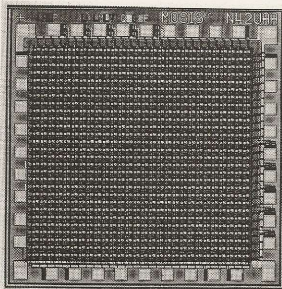
Figure 4: Micrograph of the sorting chip.
