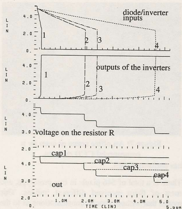
Figure 3: Sorting computational sensor: simulated operation
