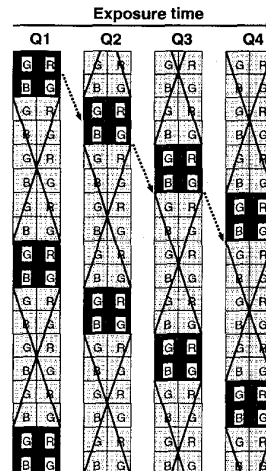
Figure 4: 'Electronic' optical low-pass filtering over four time steps (Q1...Q4) during exposure to reduce vertical aliasing in subsampled images
