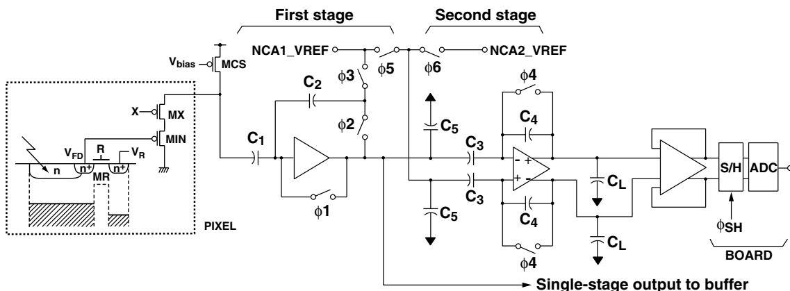
Fig. 1. Three-transistor APS and double-stage column noise canceller.
