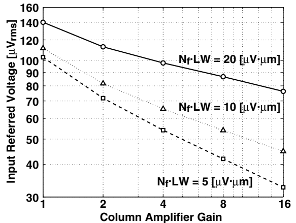
Fig. 3. Estimated input-referred noise voltage as a function of column amplifier gain.
