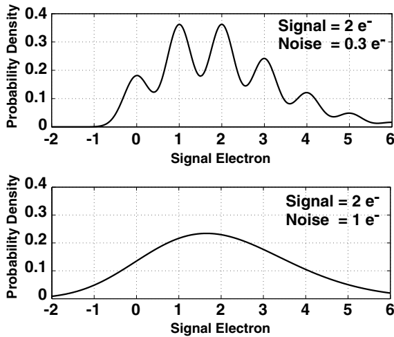
Fig. 9. Poisson distribution with circuit noise.
