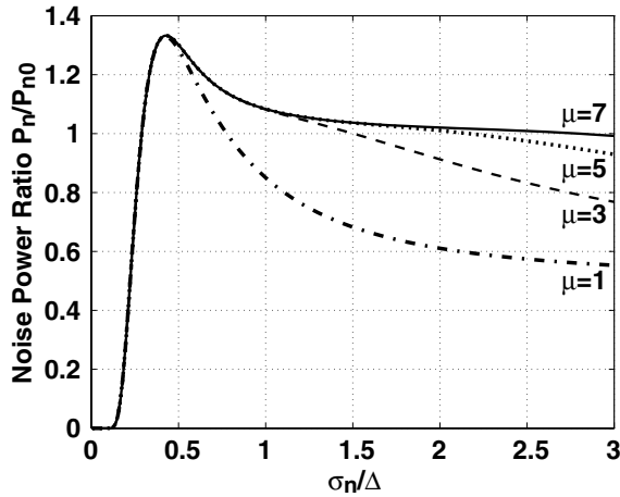
Fig. 8. Normalized noise power as a function of \sigma_n/\Delta for \mu = 1, 3, 5 and 7 .
