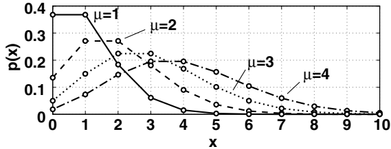
Fig. 6. Poisson distribution of photon shot noise.
