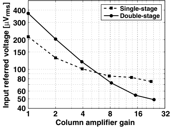
Fig. 5. Measured input-referred noise voltage as a function of column amplifier gain.
