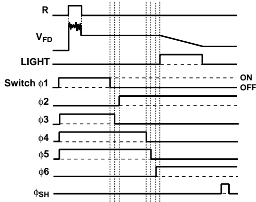
Fig. 2. Switching diagram for double-stage column noise canceller.
