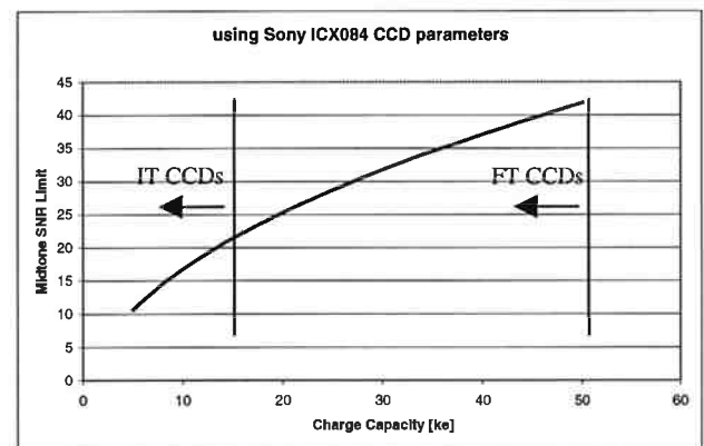
Figure 1 – Mid-tone SNR vs. Charge Capacity
