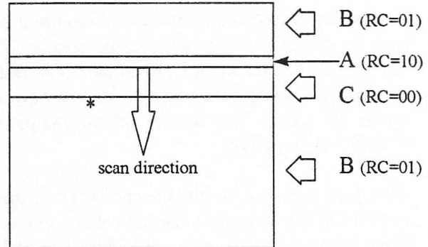
Fig. 3: Row A is being read out. All rows marked B are conditionally reset (those pixels in rows B having '1' stored in their control bit are reset on every clock). The last row B (marked *) will be read out in 1/16 of the frame time. Rows C integrate charge without any reset.
