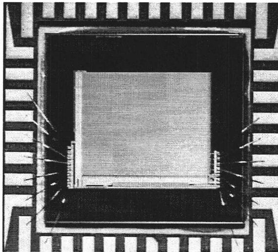
Fig. 7: 64x64 2 micron CMOS prototype chip photograph. Horizontal scan and output circuits are at the bottom, vertical scan on the left.
